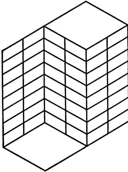
Fig. 35. — Thiéry's figure.
